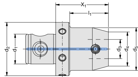
动平衡螺钉 Thread precision balancing
