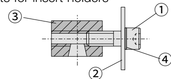
Clamping elements for insert holders
