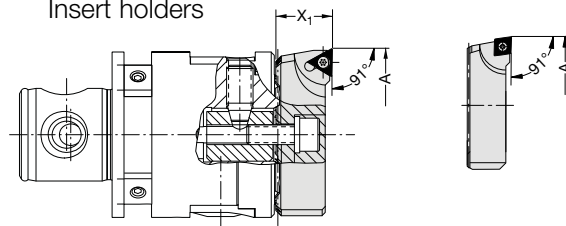
Insert holders
