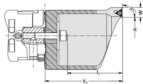
Insert holders for outside turning
